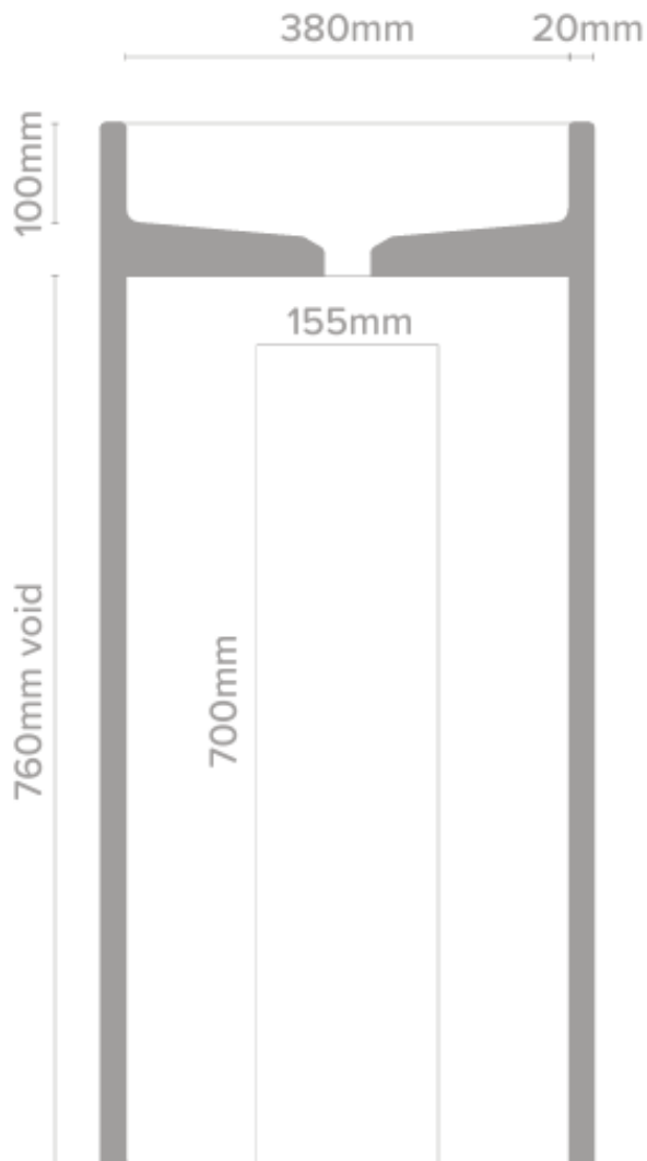
SECTION VIEW
