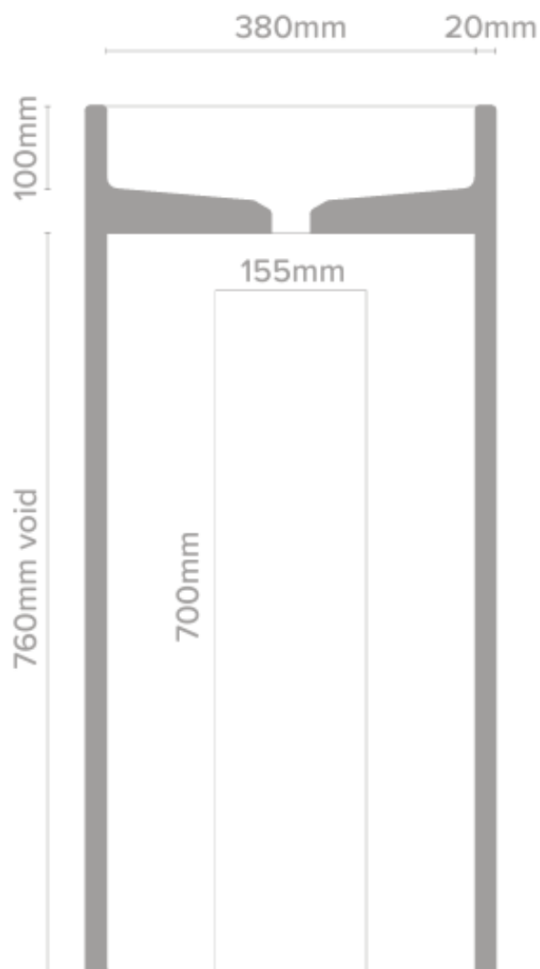
SECTION VIEW
