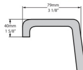
Rim Detail
