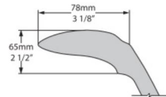
Rim Detail
