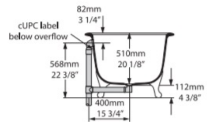
Section BB Shown with optional K50 waste kit
