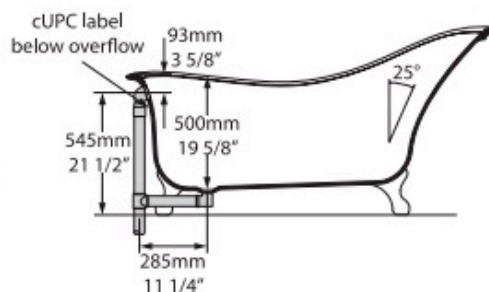
Section AA Shown with optional K50 waste kit
