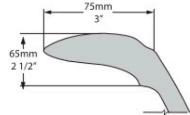
Rim Detail
